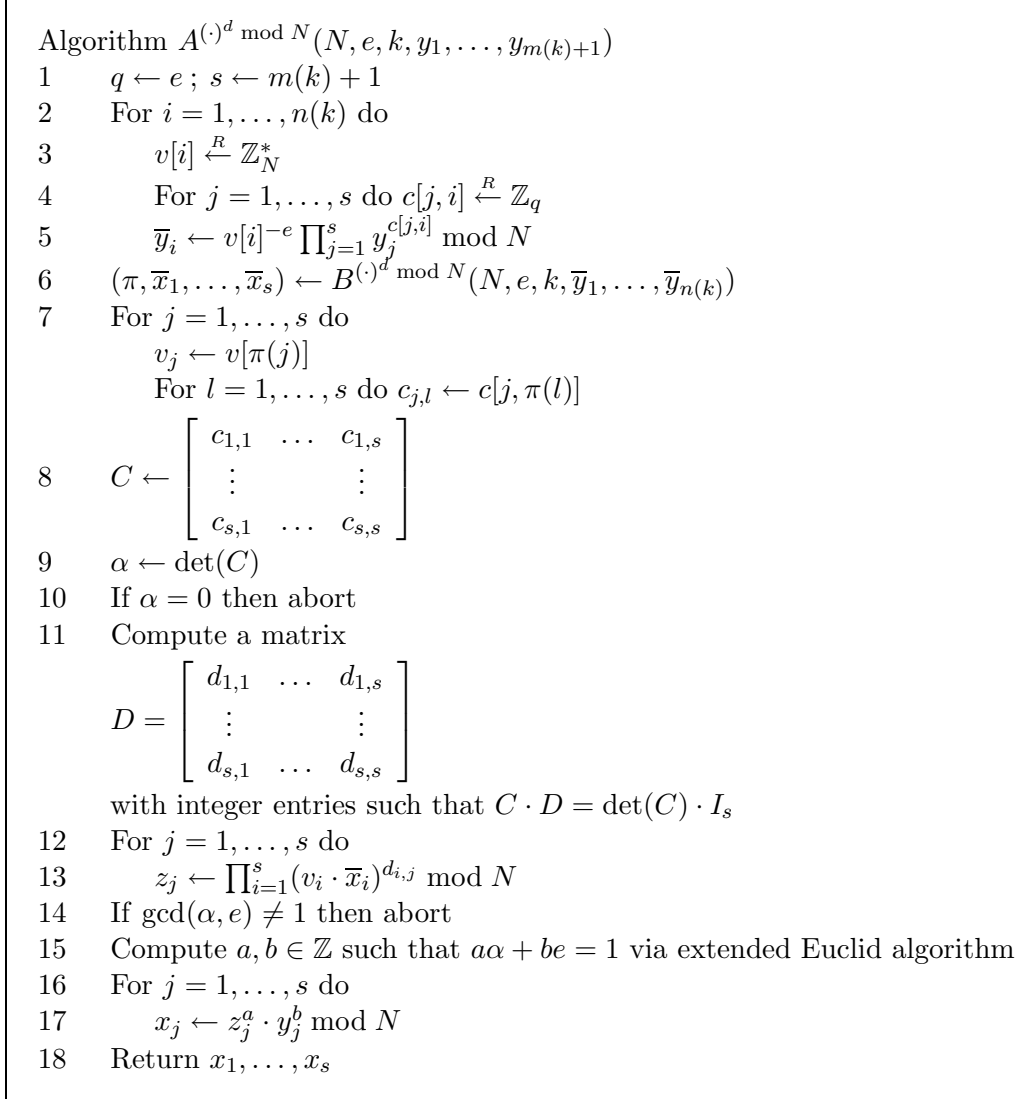
Figure 1: Adversary A of the proof of Theorem 4.1.
