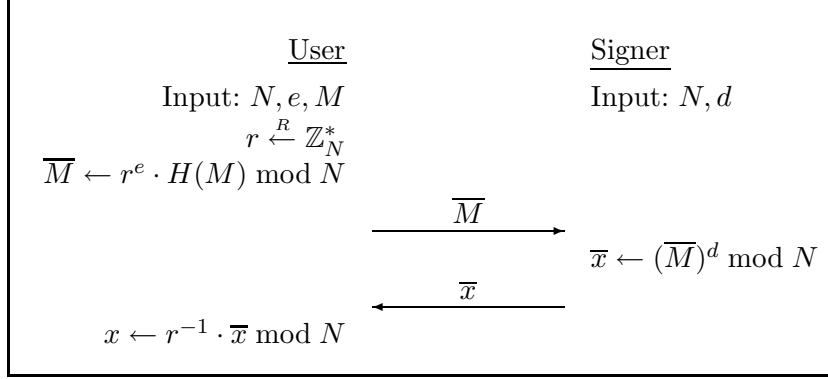
Figure 3: Blind signing protocol for FDH-RSA
