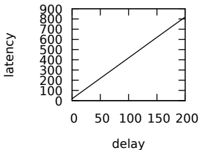
/reserve/withdraw
