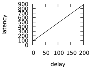
/refresh/reveal
