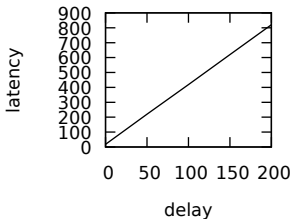
/refresh/melt
