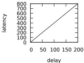
/keys
